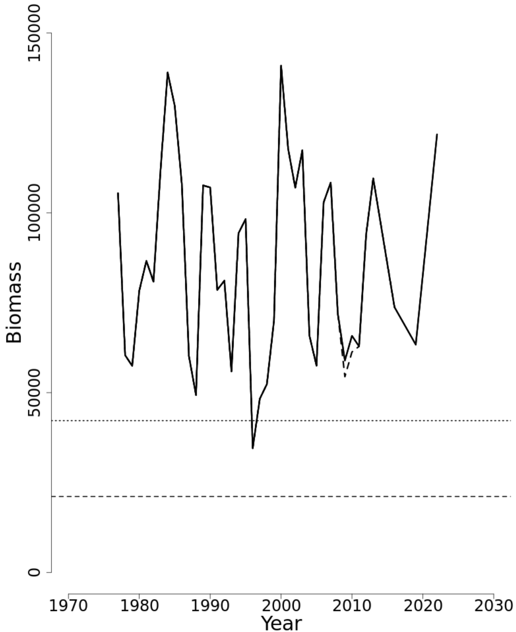
Figure 1: Trends in biomass (average of NEFSC spring and fall survey biomasses, in mt) of longfin inshore squid from the current assessment (solid line) and the 2020 assessment updates (dashed line). Biomass is the two-year moving averages of the annualized q-adjusted, swept-area biomass estimates for the NEFSC spring and fall bottom trawl surveys (i.e., annual averages of these two surveys). Biomass estimates are shown as interpolated values for years where biomass could not be estimated due to inadequate survey sampling coverage of longfin squid habitat (i.e., the 2014 and 2020 spring and 2017 and 2020 fall surveys). The approximate 80% confidence limits (106,748, 136,923) are shown for the 2022 annualized biomass estimate (121,836 mt) in relation to the annualized proxy (42,405 mt) and B_{Threshold} (21,203 mt).
