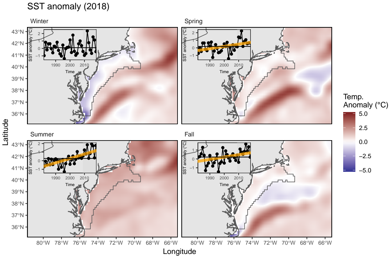
Figure 25: MAB seasonal sea surface time series overlaid onto 2018 seasonal spatial anomalies.
