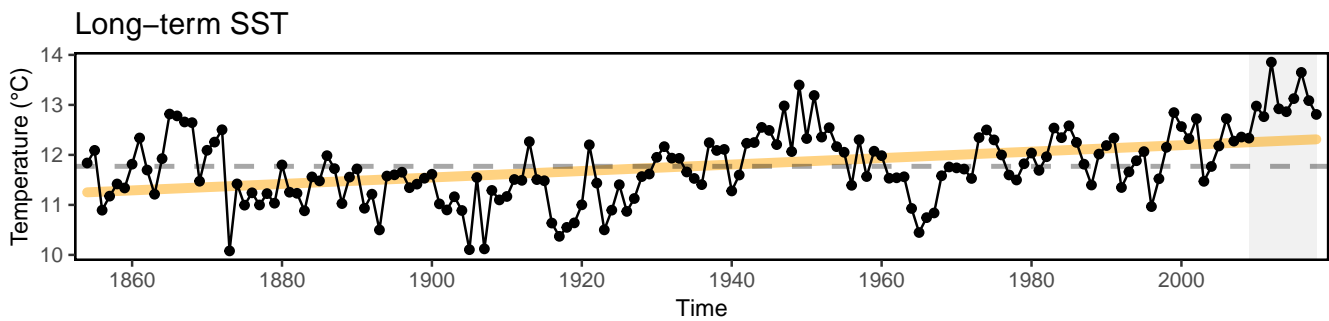
Figure 24: Average annual sea surface temperature (SST) over the Northeast US Shelf
