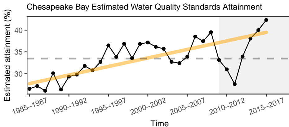
Figure 22: Estimated water quality standards attainment of Chesapeake Bay tidal waters for the combined assessment of dissolved oxygen, underwater bay grasses/water clarity and chlorophyll a using rolling three year assessment periods.
